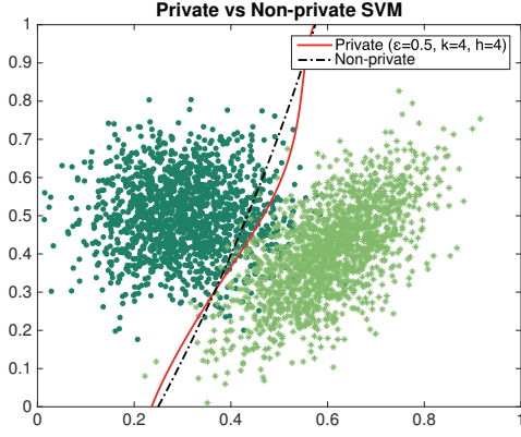
Figure 2: Private SVM with Gaussian kernel
