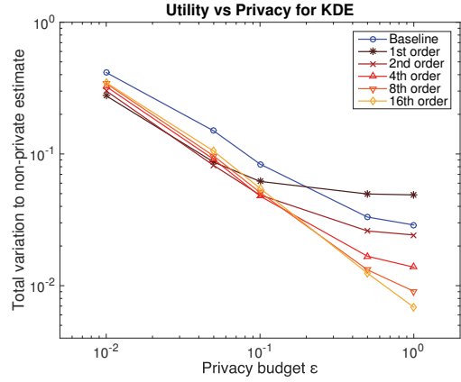
Figure 1: Private KDE with Gaussian kernel
