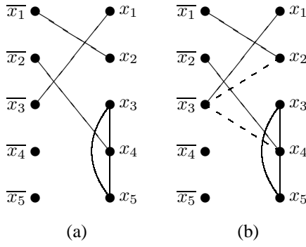
Figure 3: The split interaction graph of \Sigma_1 .
