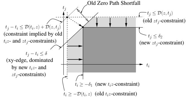
Figure 1: Reducing the zero-path shortfall for an xy-edge
