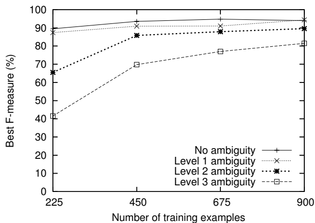
Figure 6: Learning curves for KRISPER on the AMBIG-CHILDWORLD corpus with various levels of ambiguities.
