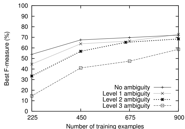
Figure 5: Learning curves for KRISPER on the AMBIG-GEOQUERY corpus with various levels of ambiguities.
