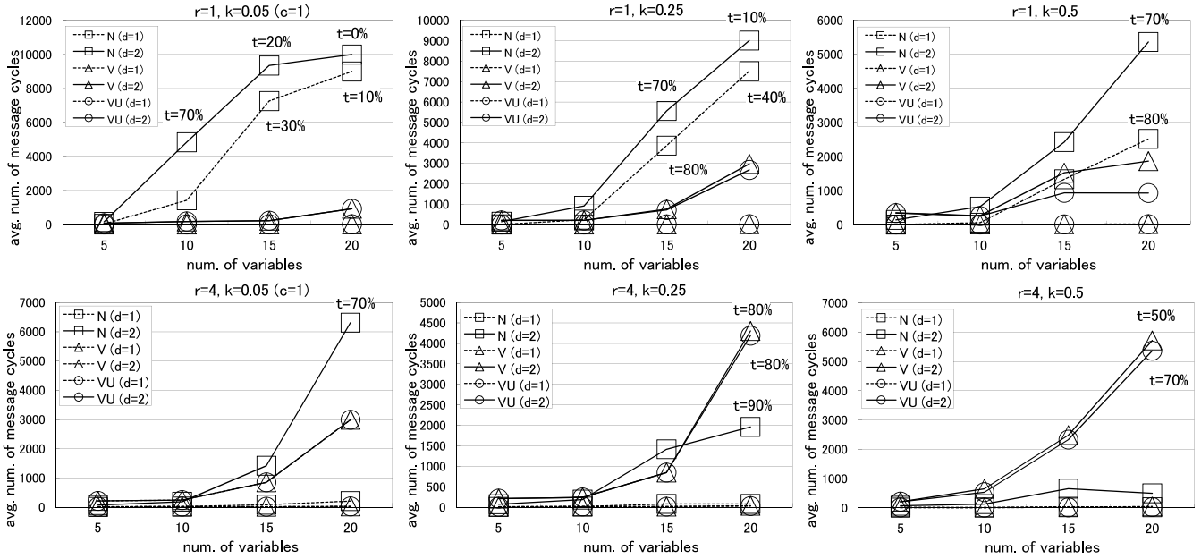
Figure 5: Message cycles (t: ratio of correctly terminated instances (others: 100%))
