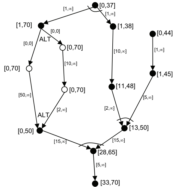
Figure 4. Domain filtering using the proposed constraint model.
