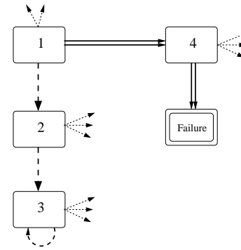
Figure 2: An example showing the utility of backjumping.
