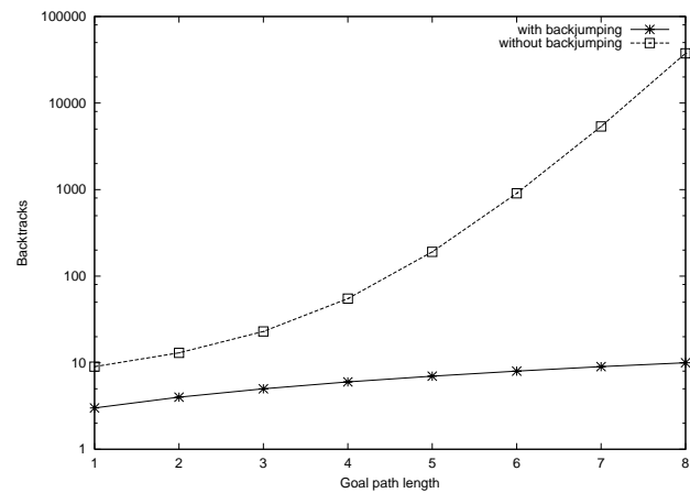
(b) Number of backtracks or backjumps [log].
