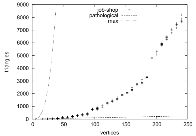
Figure 6: Relation between the numbers of vertices and triangles in our test sets
