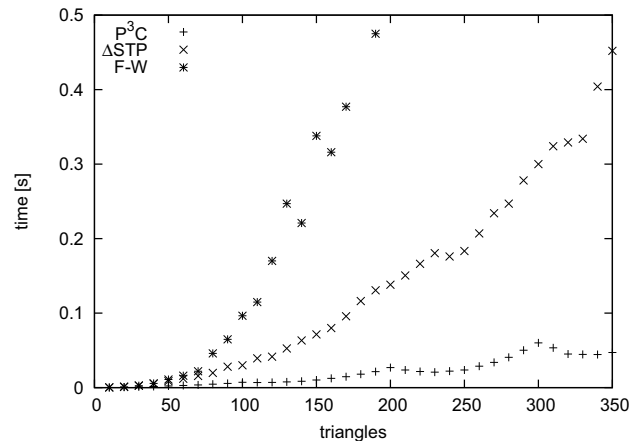
Figure 7: Performance of Floyd-Warshall, \Delta STP and P 3 C on the pathological case
