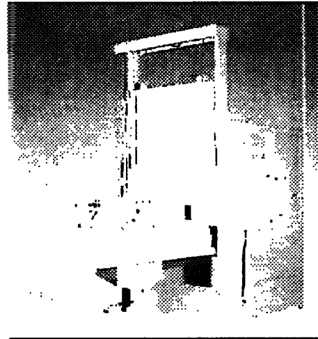
Figure 3. Flashfire burnout of RP pattern and wax gating.
