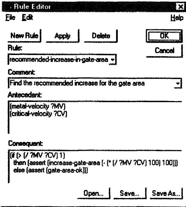
Figure 12. A view of the rule editor.
