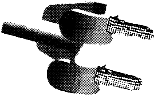
Figure 10. Point modulus visualization after adding gates. Hottest parts of the casting are in the gates.
