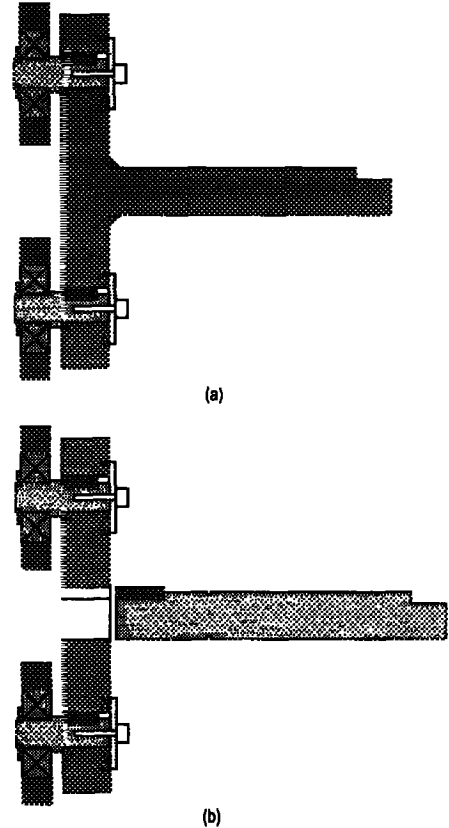
Figure 5: Two planet holder designs
