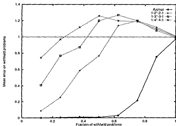
Figure 2: Generalization error (chance=1) for embodied systems and disembodied controls
