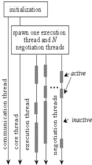
Figure 1 The basic thread architecture of our agent design
