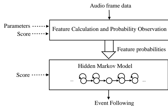
Figure 1: General diagram of IRCAM's score following
