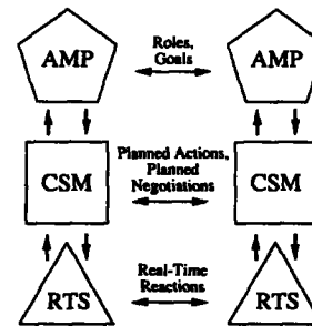
Figure 1: CIRCA agents negotiate at every level.
