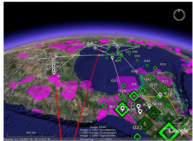
Figure 2: Google Earth with SUAs (magenta), satellite ground track (red), MOPITT/MOZART difference waypoint candidates (green diamonds), and flight plan (white).
