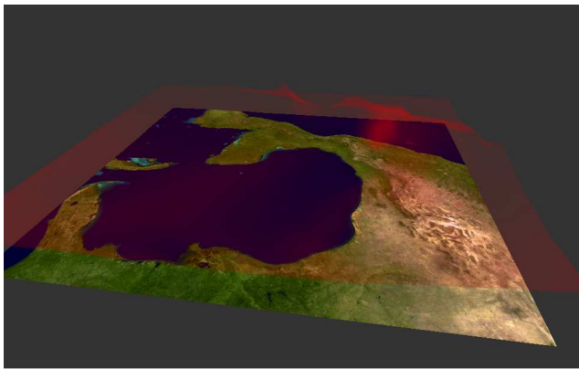
Figure 4: View of MOZART CO prediction at level 27 with 100X vertical exaggeration in Mercator.
