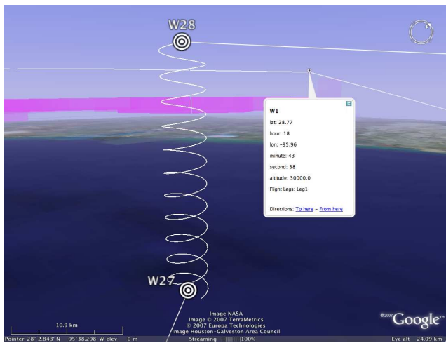
Figure 3: Detail of flight plan showing a spiral leg and attributes for a waypoint.
