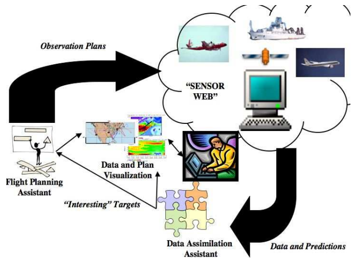
Figure 1: The daily mission flight planning cycle, integrating machine learning, visualization and flight planning.
