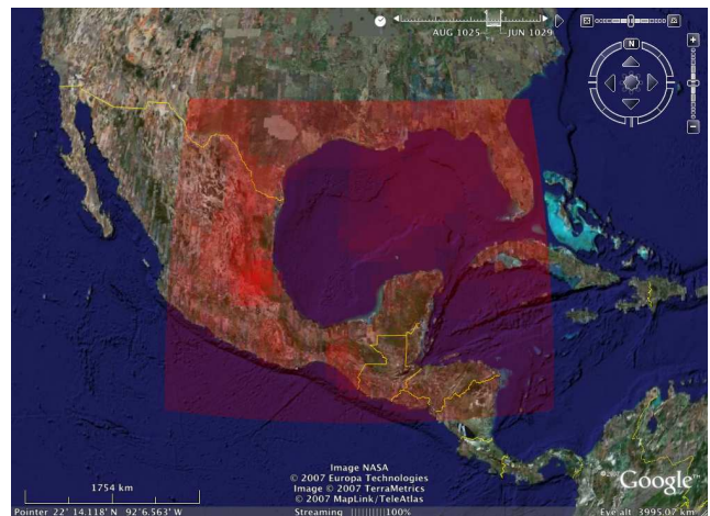
Figure 5: View of MOZART CO prediction in Google Earth.
