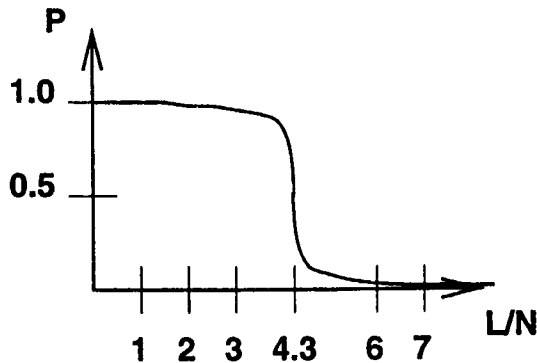
Figure 1: The transition phase for random 3SAT problems.
