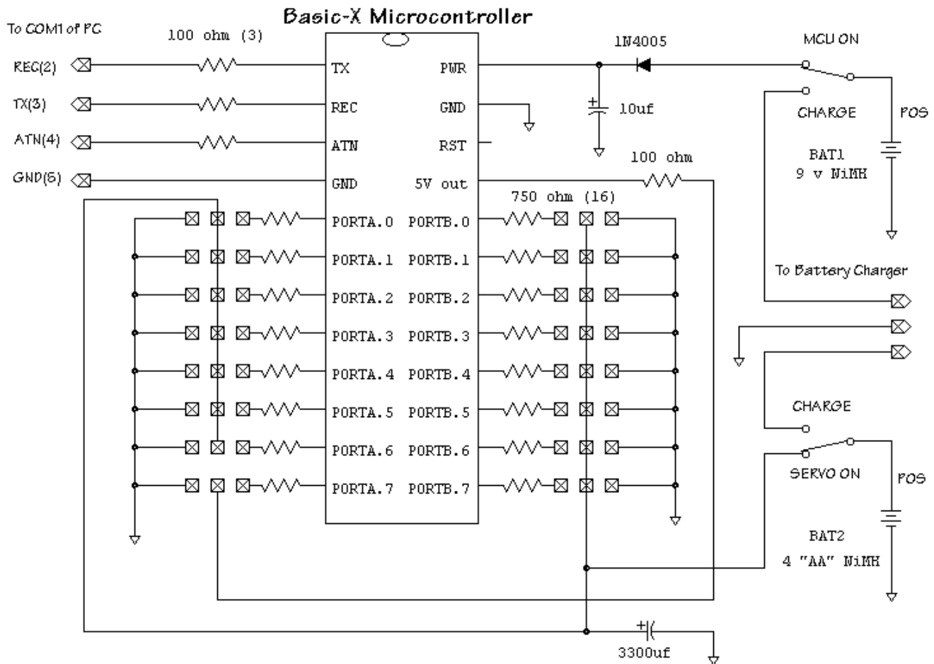
Schematic Diagram: Snake Microcontroller
