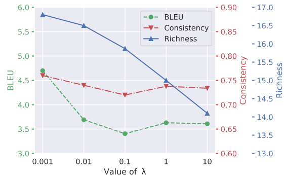
Figure 4: Impact of hyper-parameter \lambda in CNN/DailyMail.
