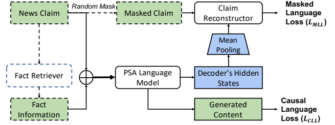
Figure 1: The proposed model, FACTGEN. The black dashed line indicates no differential dependency and the black bold line otherwise. \oplus is the text concatenation.
