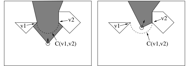
Figure 4: An example of how \phi -visibility changes when crossing a visibility curve, for \phi = \frac{\pi}{2} . As the searcher crosses C_{\frac{\pi}{2}}(v_1, v_2) , it must lose sight of at least one of v_1 and v_2 .
