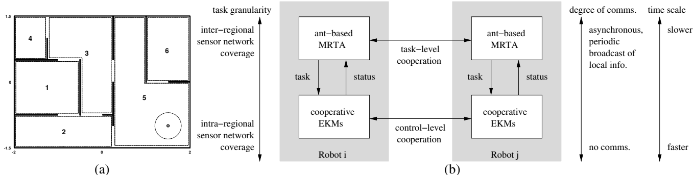
Figure 1: (a) A 4 m × 3 m environment that is divided into 6 regions. The circle at the bottom right represents the robot’s sensing radius of 0.3 m (drawn to scale). The environment is 42.44 times as large as the robot’s sensing area. (b) Two-level integrated framework for multi-robot cooperation (MRTA = Multi-Robot Task Allocation, EKM = Extended Kohonen Map).
