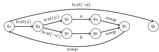
Figure 1: Automaton for \delta = \text{while } \phi \text{ do if } \psi \text{ then } a \text{ else } b . The fluent state in I_\delta represents the automaton’s state. In I_\delta ’s initial state, state = q_1 . Additional goal: state = q_8 .
