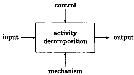
Figure 5: IDEF0 model
