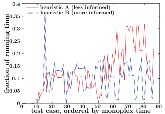
Figure 3: Fraction of running time in open stacks domain.
