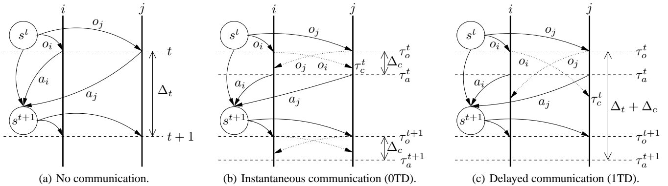
Figure 1: Illustration of different communication models used in this paper. For two consecutive time steps, and two agents, i and j , we show on what information each agent bases its action choice. In (a) we show the general Dec-POMDP setting which lacks communication. In the 0TD setting (b) agents can only decide on their actions (at \tau_a^t ) after receiving the local observation of the other agents, shortly after synchronization at \tau_c^t . Finally, (c) shows the 1TD setting, in which agents act upon receiving their local observation at \tau_a^t ( \Delta_c can be short), without waiting until \tau_c^t . However, at \tau_a^{t+1} they have received all local observations from time t , i.e., \tau_a^{t+1} > \tau_c^t .
