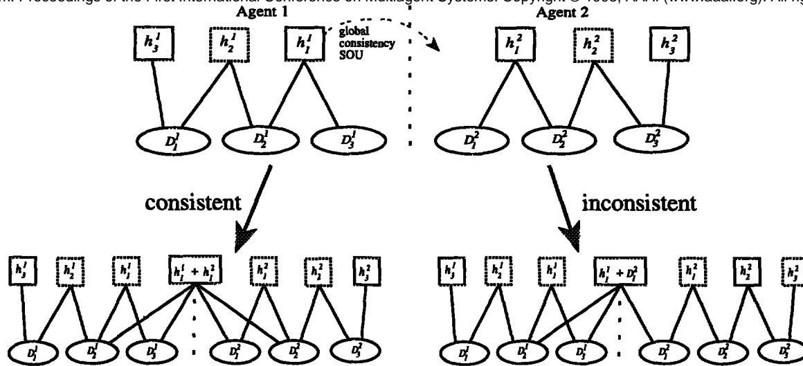
Figure 3: An example of the resolution of a global consistency SOU. When there is a consistent explanation in the external agent, resolution of the global SOU associated with h_1^1 results in the creation of a merged hypothesis as a new alternative explanation in each agent. When the local hypothesis is inconsistent with hypotheses in the external agent, new alternatives may be created (as shown here). When the local hypothesis is inconsistent with the data in the external agent, new evidential links are created to represent the contradictory evidence.
