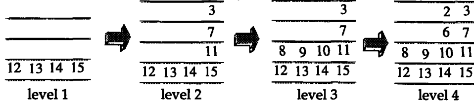
Figure 5: Serializable subgoals in n-puzzle
