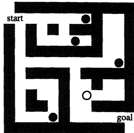
Figure 1: Search in 10×10 grid state-space (5 agents)
