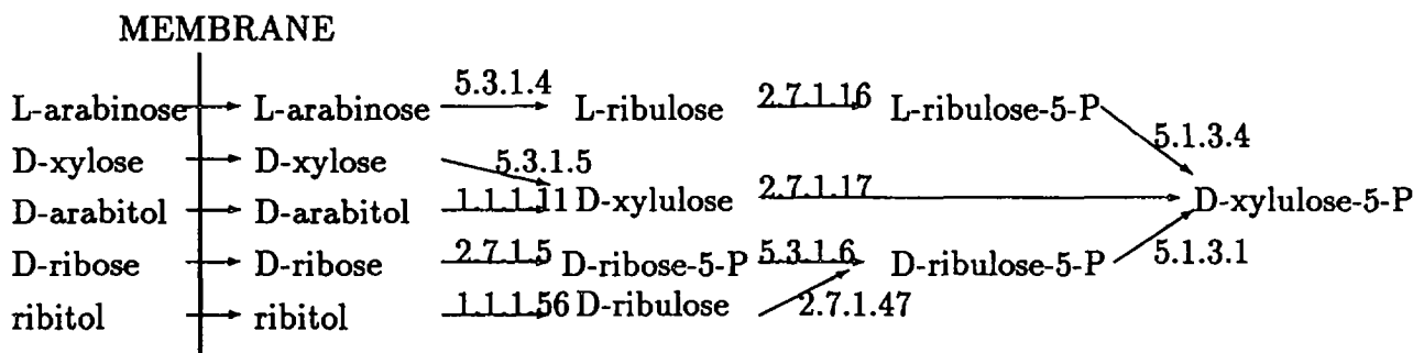
Figure 4: Pentose Pathway
