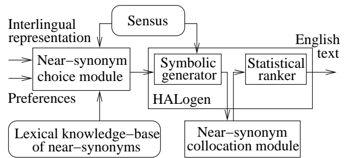
Figure 2: The architecture of Xenon.
