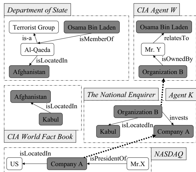
Figure 1: Discovering semantic associations from multiple documents
