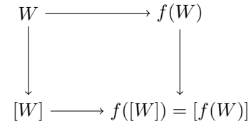
Figure 2: Orientation-consistency
