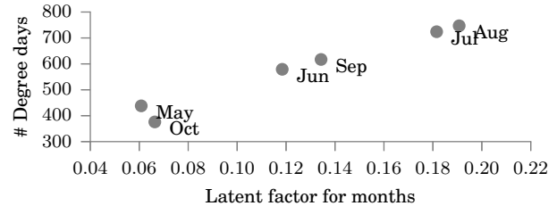
Figure 2: One of the latent factors learnt for HVAC has a high correlation with the # of degree days
