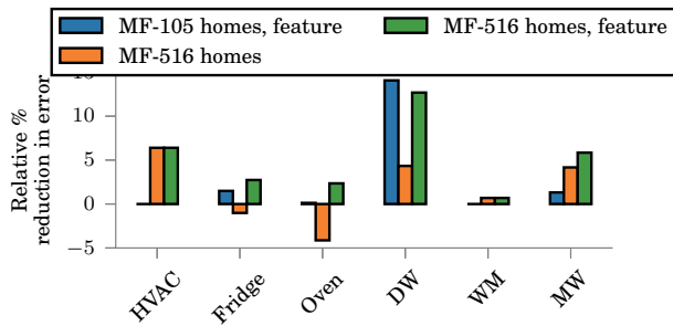
Figure 3: Reduction in error over MF on 105 homes over 6 appliances. Incorporating static features into our matrix factorisation improves energy breakdown performance.
