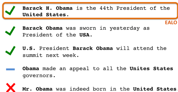
Figure 1: Sentences mentioning BARACKOBAMA and UNITEDSTATES. The EALO assumption only asserts that at least one of these expresses the fact PRESIDENTOF(BARACKOBAMA,UNITEDSTATES), when in reality 3 out of these 5 sentences actually do.
