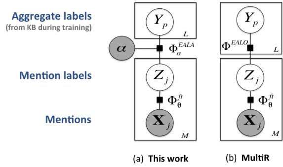
Figure 2: Graphical models for (a) this work and (b) MultiR (Hoffmann et al. 2011)
