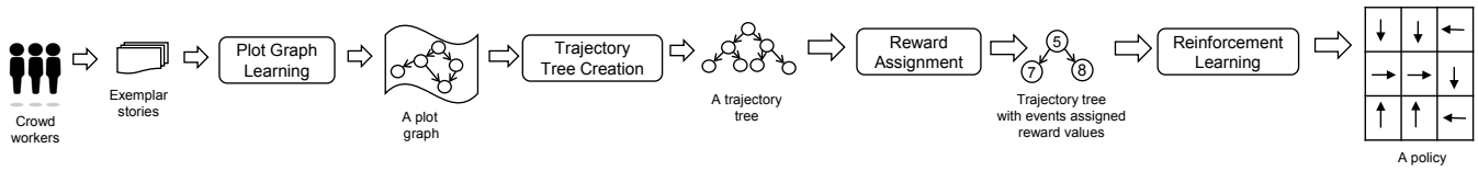
Figure 3: The process for generating value-aligned behavior from crowdsourced stories.
