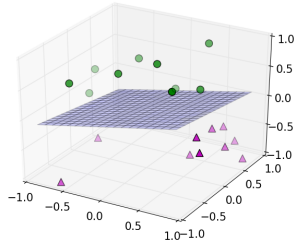
Figure 2: Model learned by certified Perceptron of Listing 4
