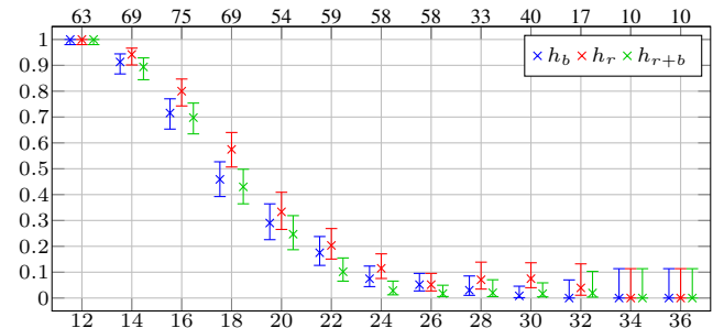
Figure 9: Coverage results as fraction of solved instances on the 15-Puzzle with time steps of 0.1 seconds. The instances are grouped by optimal plan length on the x-axis, the number of instances for each plan length is depicted at the top of the plot. The y-axis shows the fraction of solved instances with asymmetric confidence intervals of 95%.
