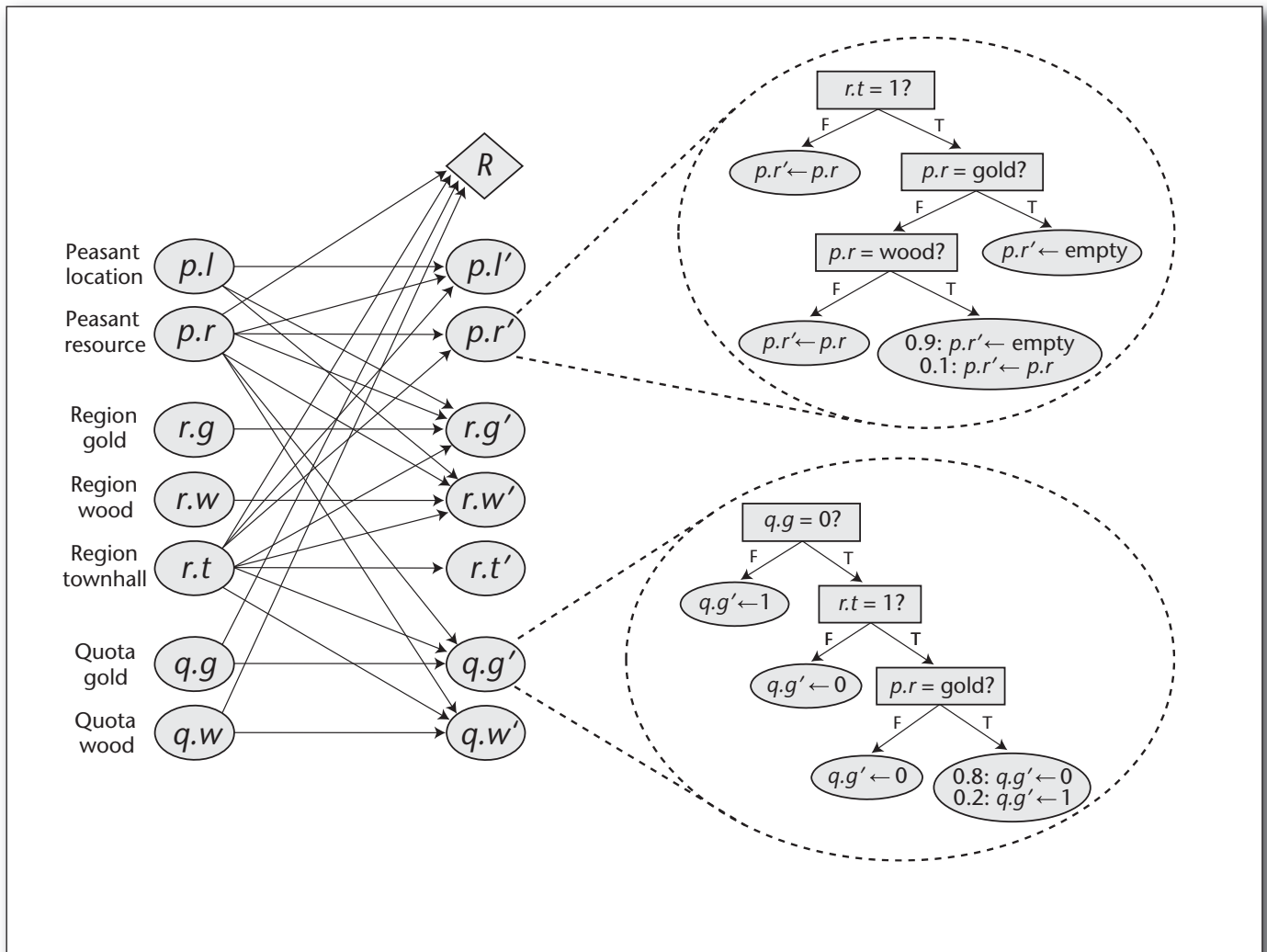
Figure 3. The Dynamic Bayesian Network Model for the Deposit Action in the Wargus Domain.
