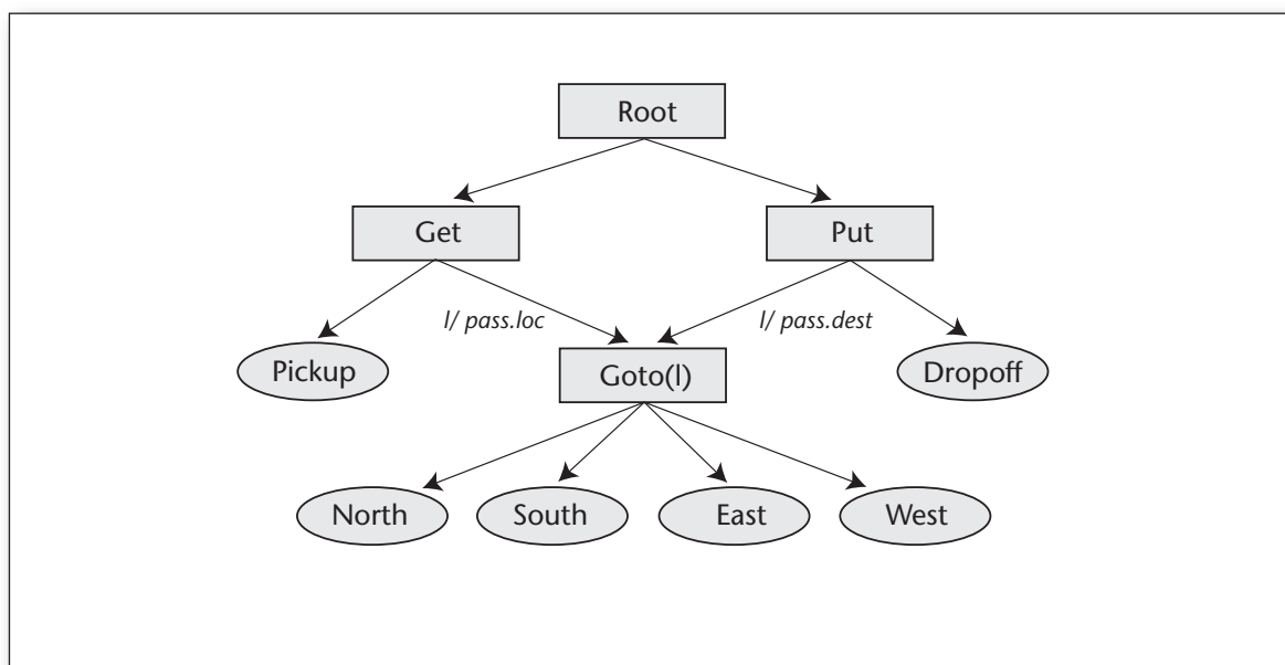
Figure 10. A Manually Designed Task Hierarchy for the Taxi Domain.
