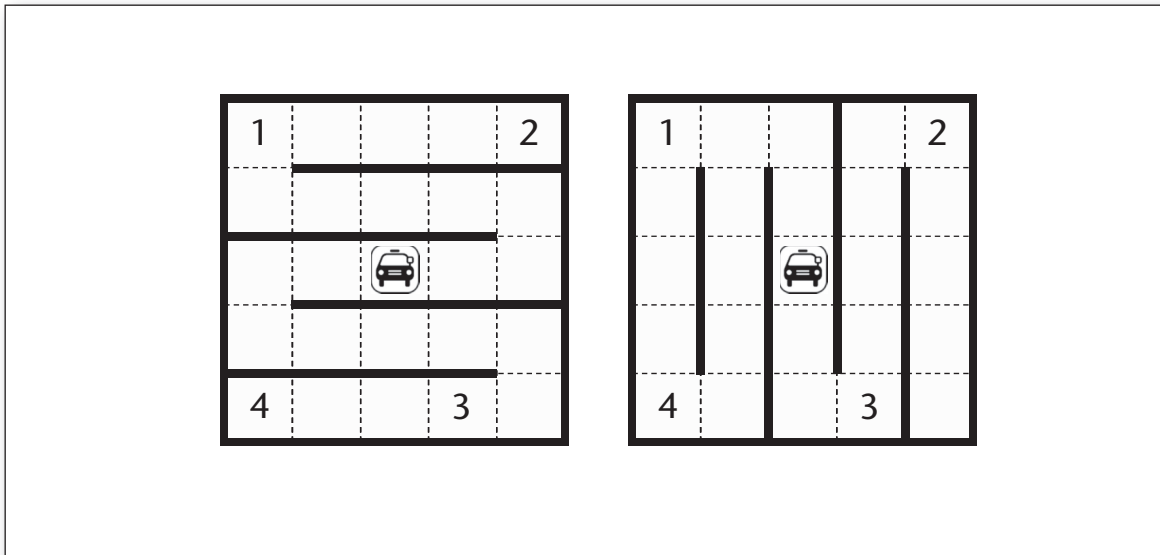
Figure 9. Source and Target Problems in the Taxi Domain.
