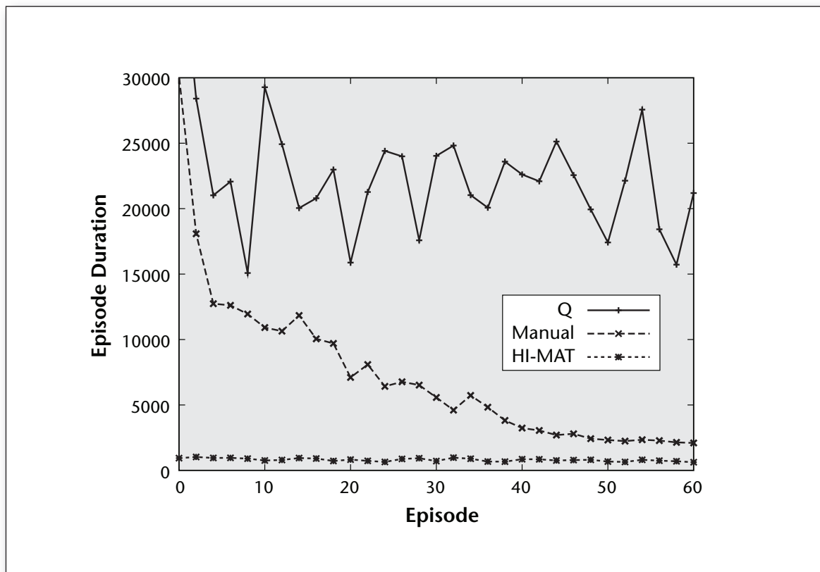
Figure 8. Performance of Three Learning Algorithms in a Target Wargus Problem (Averaged Over 10 Runs).
