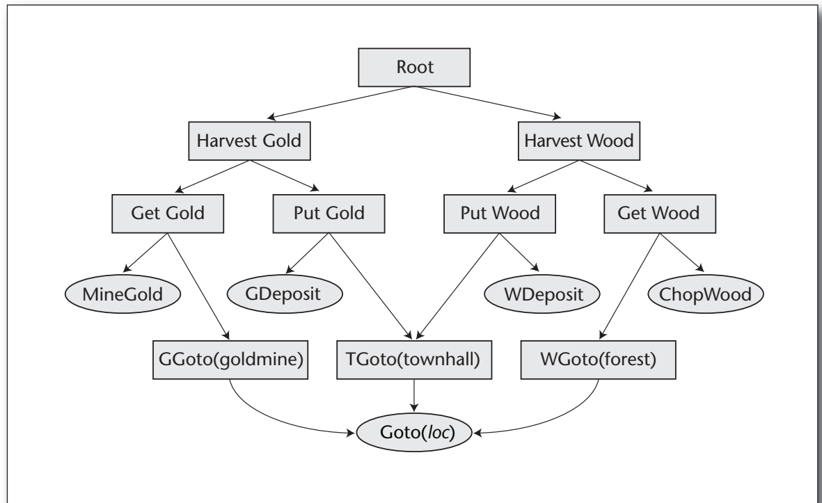
Figure 7. HI-MAT Hierarchy for Wargus.
