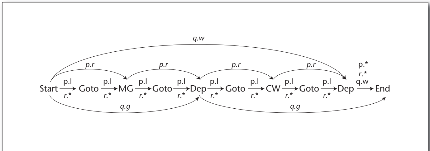
Figure 5. A CAT for the Wargus Domain.
