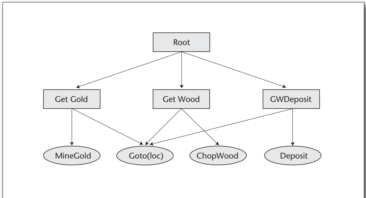
Figure 4. A Task Hierarchy for the Wargus Resource-Gathering Domain.
