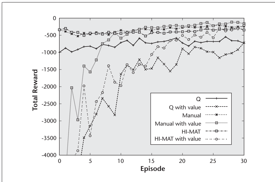
Figure 11. Performance in the Target Taxi Domain (Averaged Over 20 Runs).
