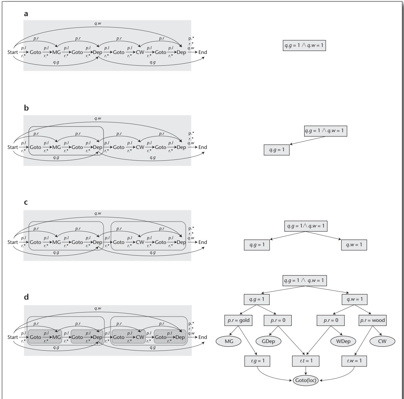
Figure 6. Illustrating the HI-MAT Algorithm in the Wargus Domain.
